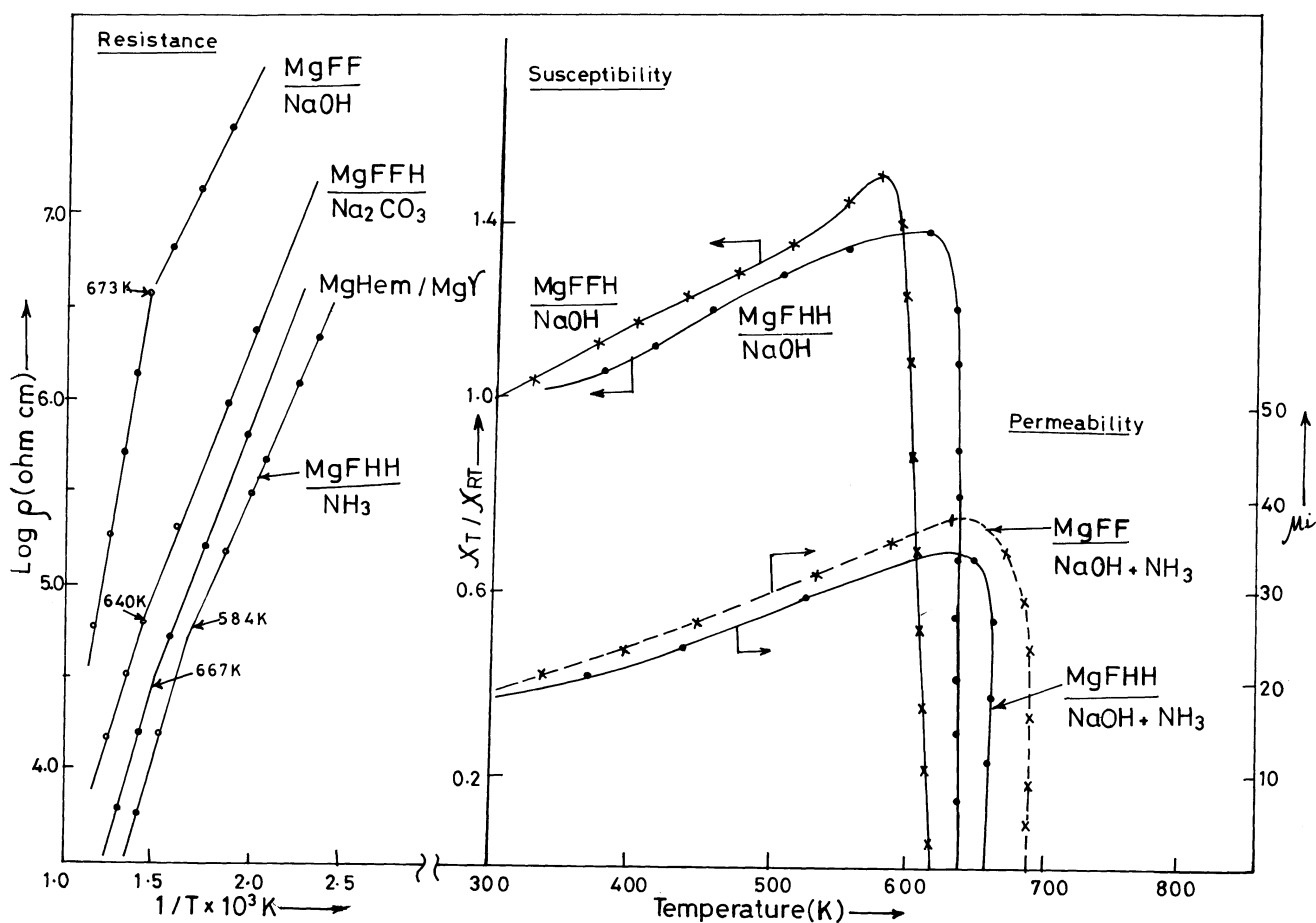
Figure 1. Temperature dependence of electrical resistivity ( r ), magnetic susceptibility ( C_T/C_{RT} ) and initial permeability ( \mu_i ) of MgFe_2O_4 .
