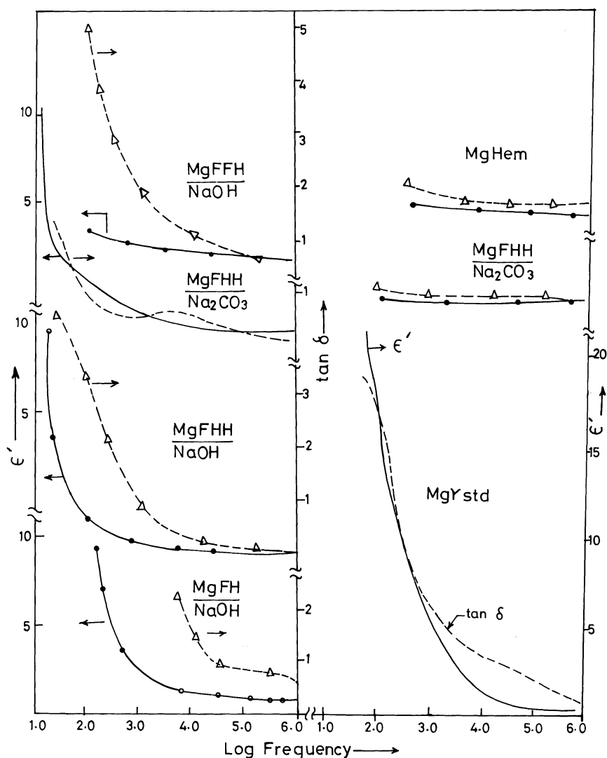
Figure 2. Frequency dependence of dielectric constant ( \epsilon' ) and \tan d loss of MgFe_2O_4 .
