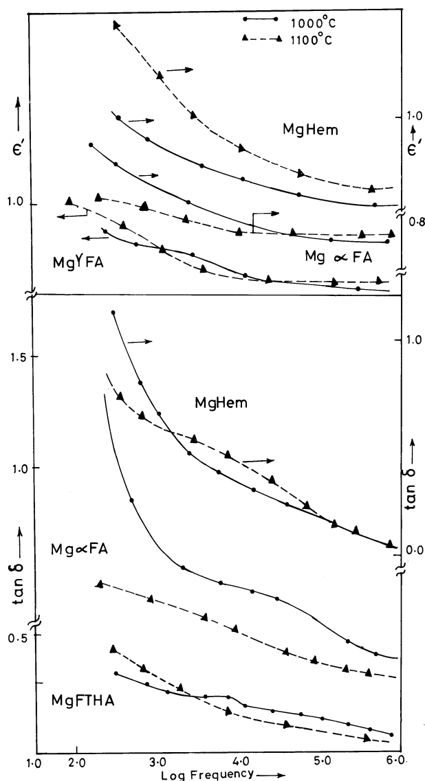
Figure 3. Effect of sintering on the dielectric behaviour of \text{MgFe}_2\text{O}_4 .
