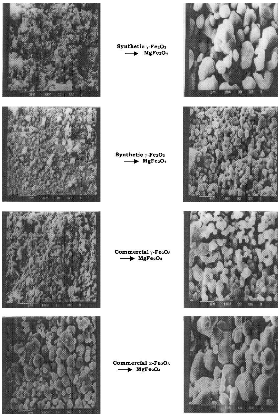
Figure 4. SEM micrographs of iron oxides and MgFe_2O_4 .
