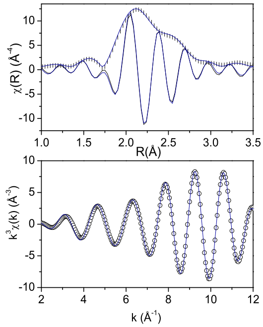
FIG. 8: (Color online) Magnitude and real component of FT of EXAFS spectra in R space and real component of FT in the back transformed k space for Ni K-edge in \text{Ni}_{50}\text{Mn}_{35}\text{Sn}_{15} obtained at low temperature. Fit to the data are shown as coloured lines.
