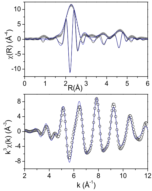
FIG. 6: (Color online) Magnitude and real component of FT of EXAFS spectra in R space and real component of FT in the back transformed k space for Mn K-edge in \text{Ni}_{50}\text{Mn}_{35}\text{Sn}_{15} obtained at room temperature. The fitting to the data are shown as coloured lines.
