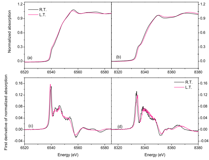
FIG. 9: (Color online) Near edge structure at the Mn K-edge (a) and Ni K-edge (b) in the austenitic and martensitic phases in \text{Ni}_{50}\text{Mn}_{35}\text{Sn}_{15} . The first derivative of the near-edge spectra are also shown for Mn K-edge (c) and Ni K-edge (d) at room temperature and low temperature
