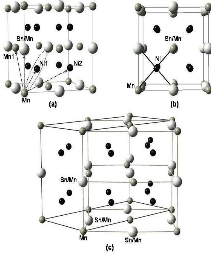
FIG. 4: (Color online) The crystal structure of \text{Ni}_{50}\text{Mn}_{35}\text{Sn}_{15} based on which the EXAFS have been modeled. (a) The L2_1 cubic phase shows the absorbing atom and the relevant backscatters. The arrows indicate different SS paths while the dotted loop shows the MS path. (b) The plane of atoms in the cubic crystal represents the fact that Y-Mn and Sn/Z-Mn are equidistant from Ni. (c) The Pmma crystal structure in the martensitic phase wherein the L2_1 type atomic arrangement is visualized.
