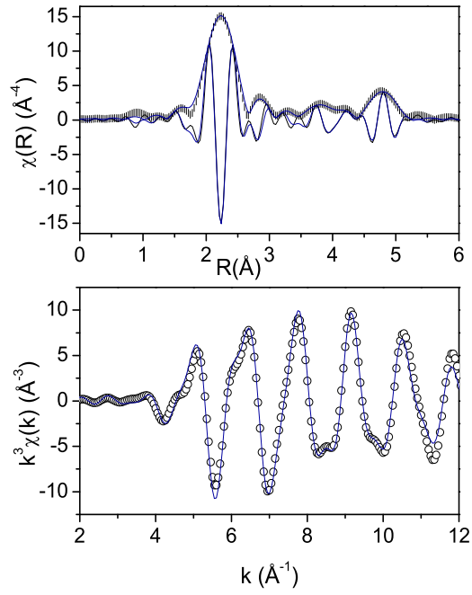
FIG. 7: (Color online) Magnitude and real component of FT of EXAFS spectra in R space and real component of FT in the back transformed k space for Mn K-edge in \text{Ni}_{50}\text{Mn}_{35}\text{Sn}_{15} obtained at low temperature. Coloured lines represents the fit to the data.
