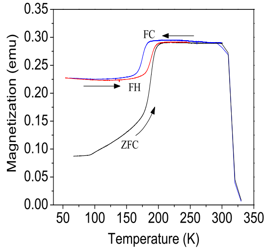
FIG. 2: (Color online) Temperature dependence of magnetization of \text{Ni}_{50}\text{Mn}_{35}\text{Sn}_{15} measured in an applied field of 50 Oe between 50 to 350 K. Measurements were carried out while heating (ZFC), cooling (FC) and re-heating (FH) the sample as indicated by the arrows. The structural and magnetic transition temperatures were determined from the differentials of magnetization with respect to temperature for FC and FH curves.
