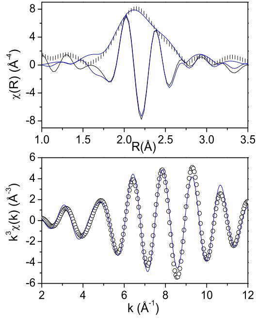
FIG. 5: (Color online) Magnitude and real component of FT of EXAFS spectra in R space (top panel) and real component of FT in the back transformed k space (bottom panel) for Ni K-edge in \text{Ni}_{50}\text{Mn}_{35}\text{Sn}_{15} obtained at room temperature. The fitting to the data are shown as coloured lines.
