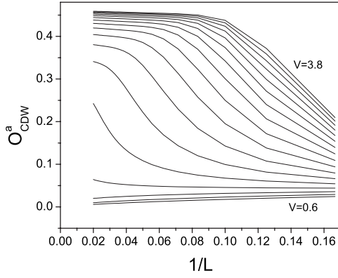
FIG. 4. Plot of CDW order parameter O_{\text{CDW}}^a for a -type atoms as a function of 1/L for values of V ranging from 0.6 to 3.8 in steps of 0.2. The O_{\text{CDW}}^a goes to zero for V < V_C \approx 1.2 whereas it is nonzero for higher values of V which shows the transition to CDW phase at V_C \approx 1.2 .
