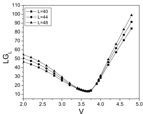
FIG. 7. The scaling of gap LG_L is plotted as a function of V for different system sizes for \Delta U=1.05 , \Delta V=1.25 , and U=6 . Coalescence of different plots between 3.4 < V < 3.9 shows a gapless PSSF phase sandwiched between PSMI and PSCDW phases.
