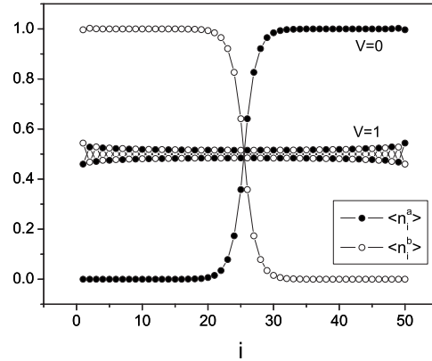
FIG. 2. Plots of \langle n_i^a \rangle and \langle n_i^b \rangle versus i for V=0 and 1 , respectively, showing PSMI and MI phases.
