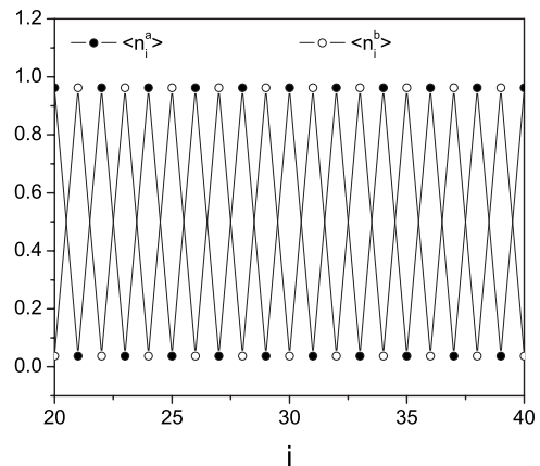
FIG. 3. Plots of \langle n_i^a \rangle and \langle n_i^b \rangle versus i for V=4 showing intermingled CDW phases for a and b types of bosons.
