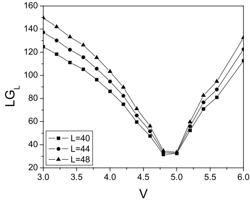
FIG. 6. Scaling of gap LG_L is plotted as a function of V for different system sizes for \Delta U=1.05 , \Delta V=1.25 , and U=9 . The gaps remain finite for all the values of V and shows the PSMI-PSCDW transition with V_C \approx 4.7 .
