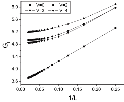
FIG. 1. Gap G_L versus 1/L for different values of V for U=9 , \Delta U=1.05 , and \Delta V=0.5 . G_{L \rightarrow \infty} converges to a finite valued signaling Mott-insulator phase.
