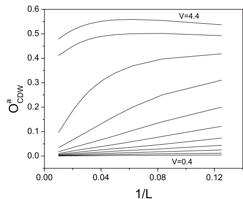
FIG. 9. Plot of O_{CDW}^a as a function of 1/L for values of V ranging from 0.4 to 4.4 in steps of 0.4.
