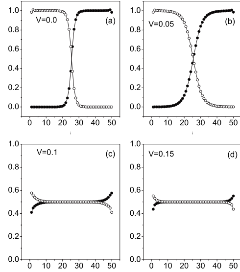
FIG. 5. Density distributions for different values of V with \Delta V=0.5 , U=6.0 , and \Delta U=1.05 .
