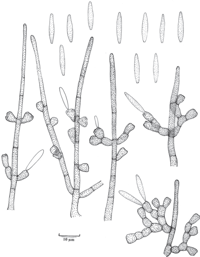
FIG. 3. Spondylocladiopsis aseptata . Conidiophores with conidiogenous cells and conidia.
