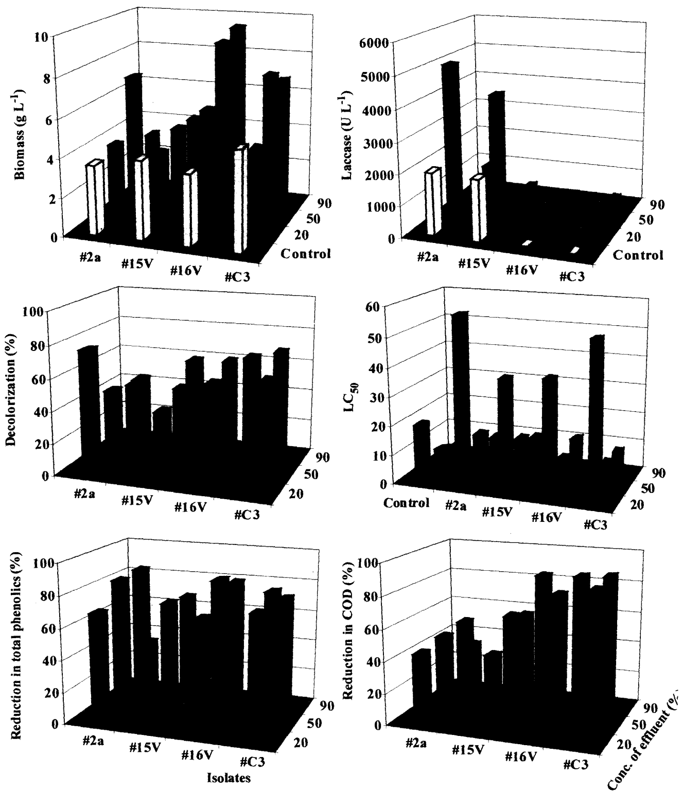
Fig. 3.10: Response of fungi in the presence of TEB added at 20% (lightest), 50% (medium) and 90% (darkest) to 6-day old cultures (in situ). Controls: □ Without any effluent, ■ Only TEB in the medium without any culture.
