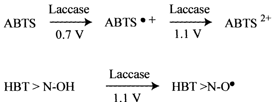
Fig. 3.2: Redox potentials of the oxidation reactions of ABTS and HBT by laccase. Adapted from: Kunamneni et al., 2008
