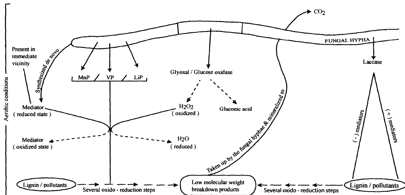
FIG. 1. Schematic diagram illustrating the role and activity of various extracellular lignin-degrading enzymes produced by fungi (Modified from Field et al. 1993). MnP = manganese-dependent peroxidase; LiP = lignin peroxidase; VP = versatile peroxidase.
