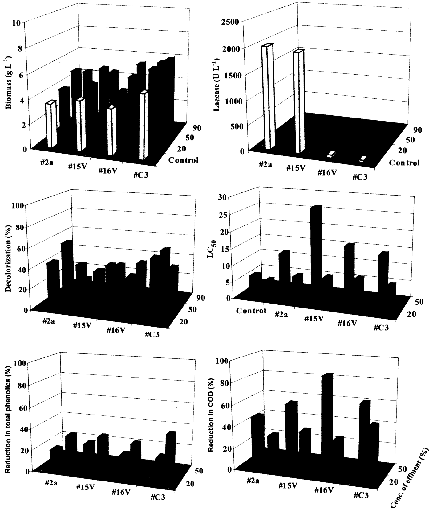
Fig. 3.9: Response of fungi in the presence of TEA added at 20% ■, 50% ■ and 90% ■ to 6-day old cultures (in situ) Controls: □ Without any effluent, ■ Only TEA in the medium without any culture.
