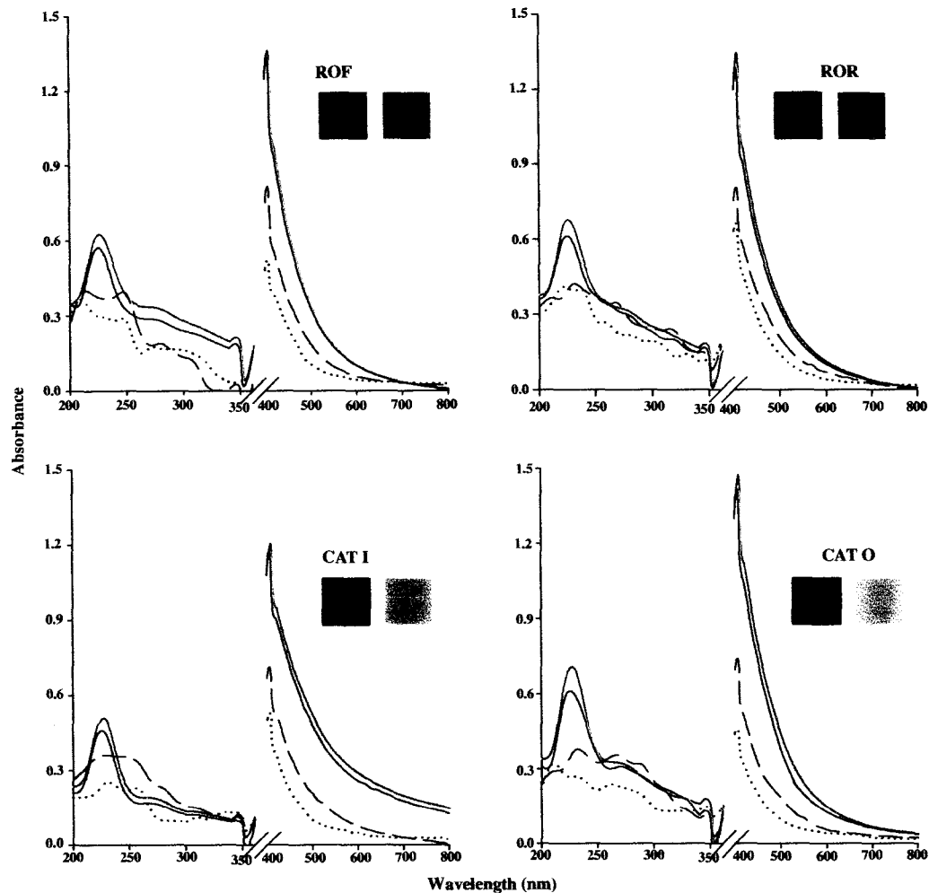
Fig. 1. Visible and UV spectra of the four effluents; untreated (—), after sonication (---), after treatment with the whole fungus (· · ·) and after biosorption with wet, heat-killed biomass (- · - ·). The UV and visible spectra were taken at different dilutions. The insets indicate the initial and final colors of the effluents.
