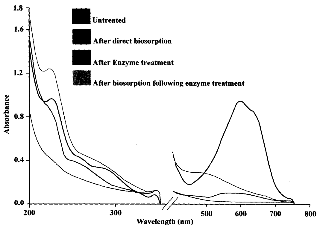
Fig. 3.23: Visible and UV spectra of the Reactive Blue 4; Untreated (—), after direct biosorption (---), after enzymatic treatment (····) and after enzymatic treatment followed by biosorption (-·-·). The insets indicate colors of untreated dye and after each step of treatment.
