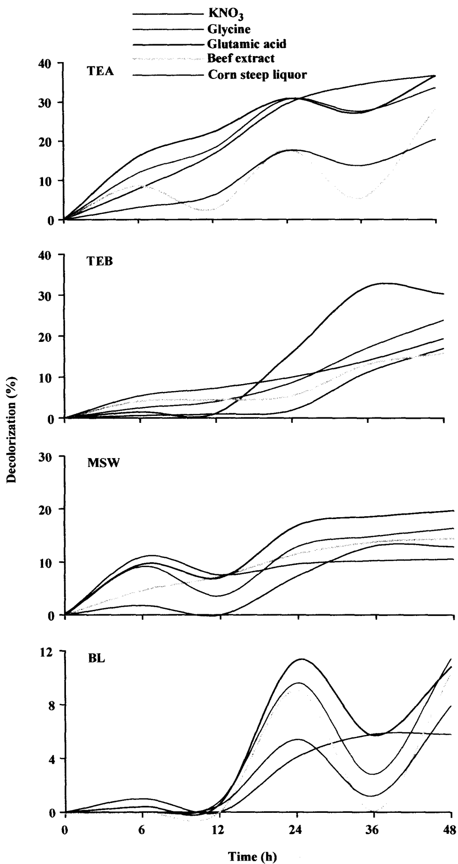
Fig. 3.5: In vitro decolorization of effluents with 1000 color units each using 10U of crude laccase obtained from different nitrogen sources namely, KNO 3 , Glycine, Glutamic acid, Beef extract and Corn steep liquor. Decolorization was monitored from 0 to 48 h. The standard deviation values were less than 10%.
