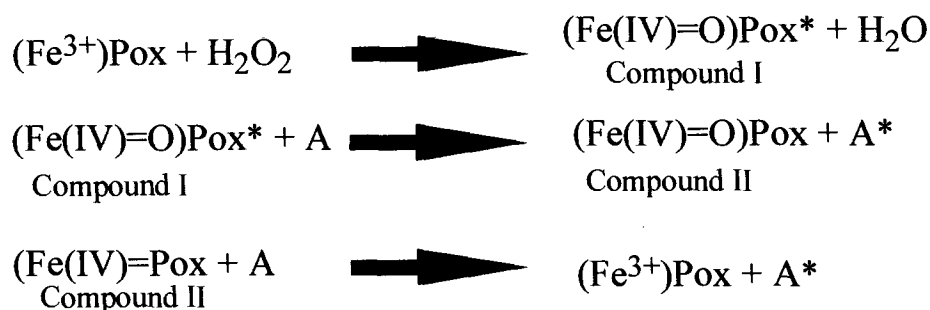
Fig. 1.3: Reaction mechanism for heme peroxidases. The hemeperoxidase is a redox process consisting of three distinct steps. The first step is the reaction of the resting enzyme [(Fe 3+ )Pox] with H 2 O 2 in a two electron transfer which results in the formation of Compound I. Compound I has one reducing equivalent at the oxyl-ferric iron [Fe(IV)=O] and the other forms a cation radical [Pox*]. Compound I is then reduced by the substrate (A) in two sequential one-electron steps through Compound II. Adapted from: Conesa et al. 2002.
