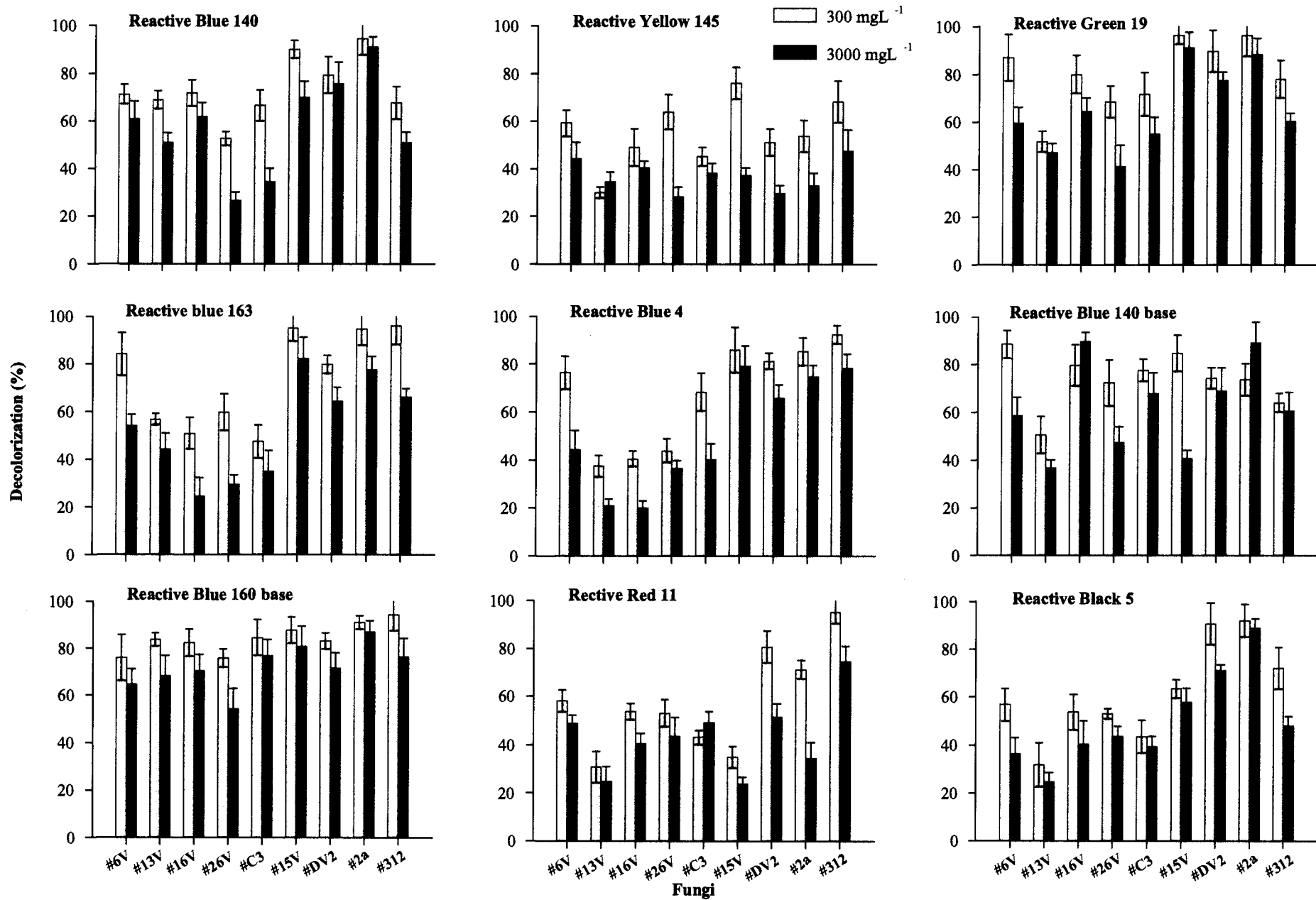
Fig. 2.10: Decolorization of reactive dyes at two different concentrations using various isolates, estimated on day 3, 6 and 9. NIOCC #2a and #312 were used as reference isolates.
