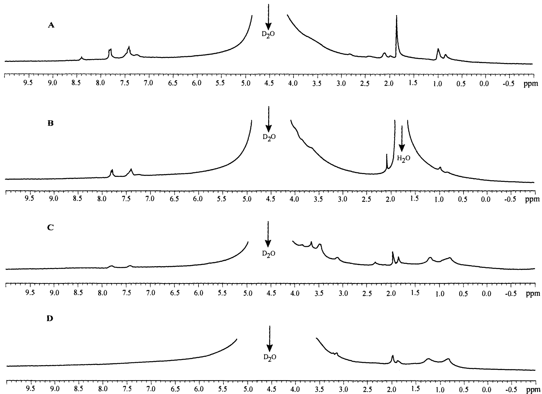
Fig. 3.20: ^1\text{H} NMR spectra A) untreated CAT O; B) after Step 1-sonication; C) after Step 2- whole fungus treatment; D) after Step 3- biosorption.
