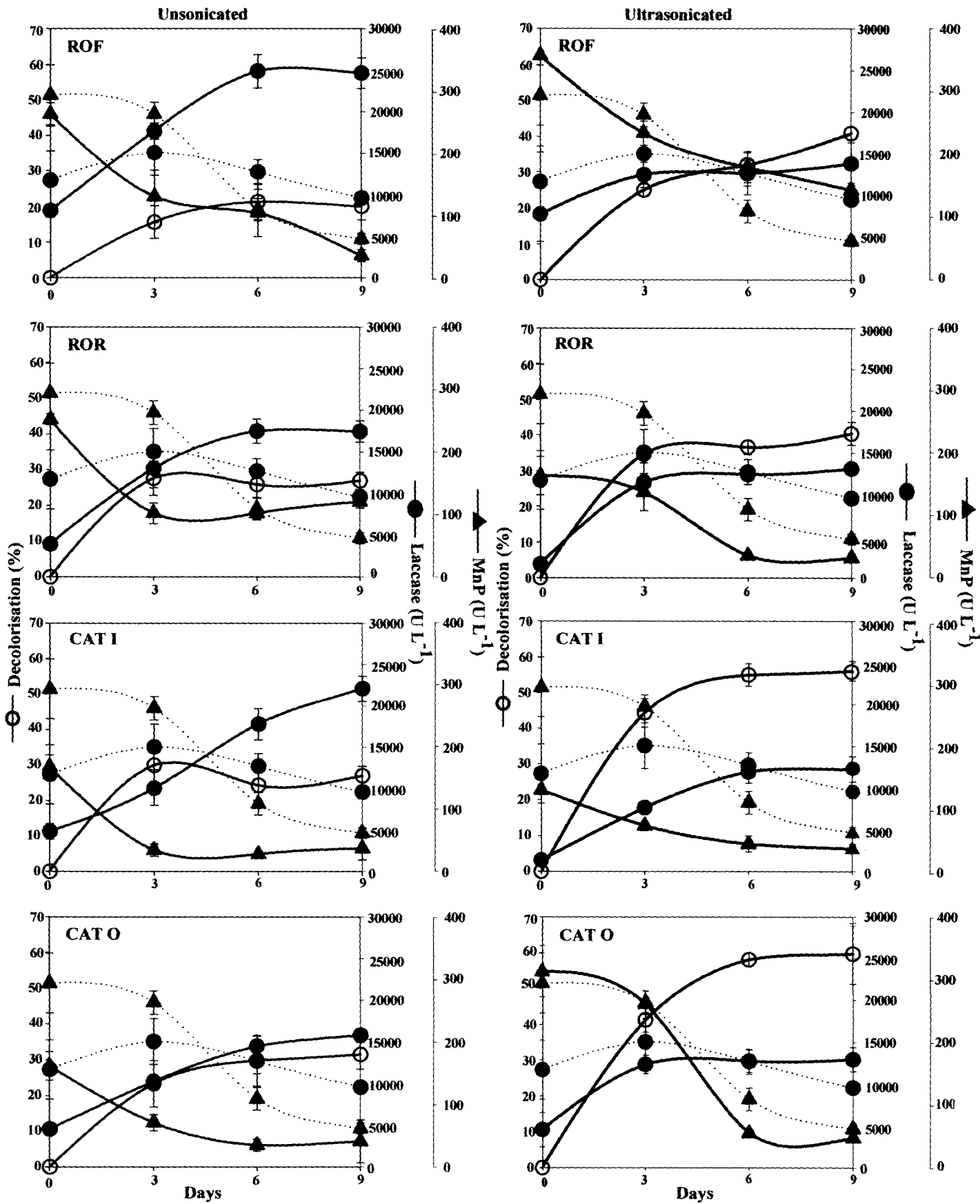
Fig. 3.17: Decolorization, laccase and MnP production by NIOCC #2a in LN medium during whole-fungal culture treatment (Step 2). Four graphs on the left are with unsonicated effluents (—), and the four graphs on the right are with ultrasonicated effluents (—). Laccase and MnP production in the control culture, without any effluents are shown by dotted lines (—) in all the graphs.
