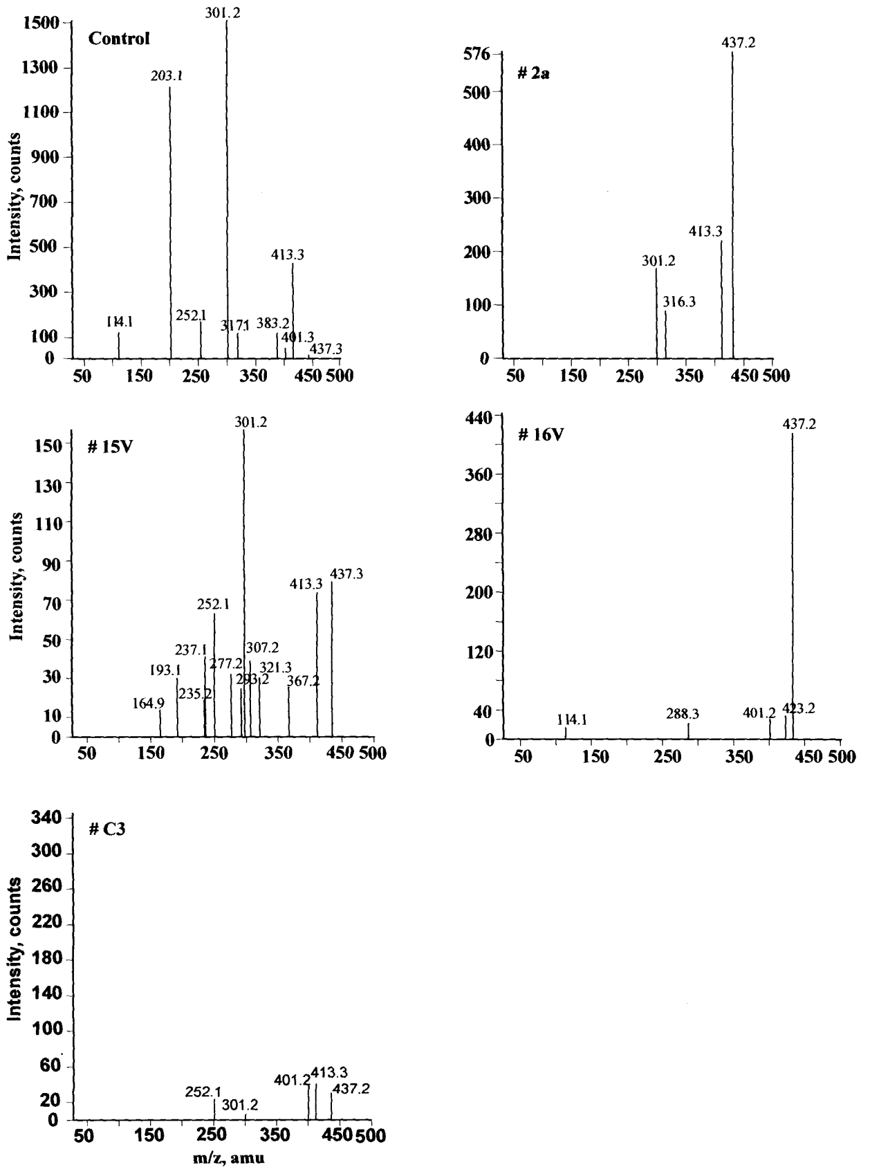
Fig. 3.13: Electrospray ionization mass spectra with characteristic ions related to specific low mass ions were recorded at 0-1,000 m/z in positive mode. Mass spectra of untreated (control) and fungal-treated (in situ) TEB. Note the difference in intensity counts (Y axis) in various cultures and the control
