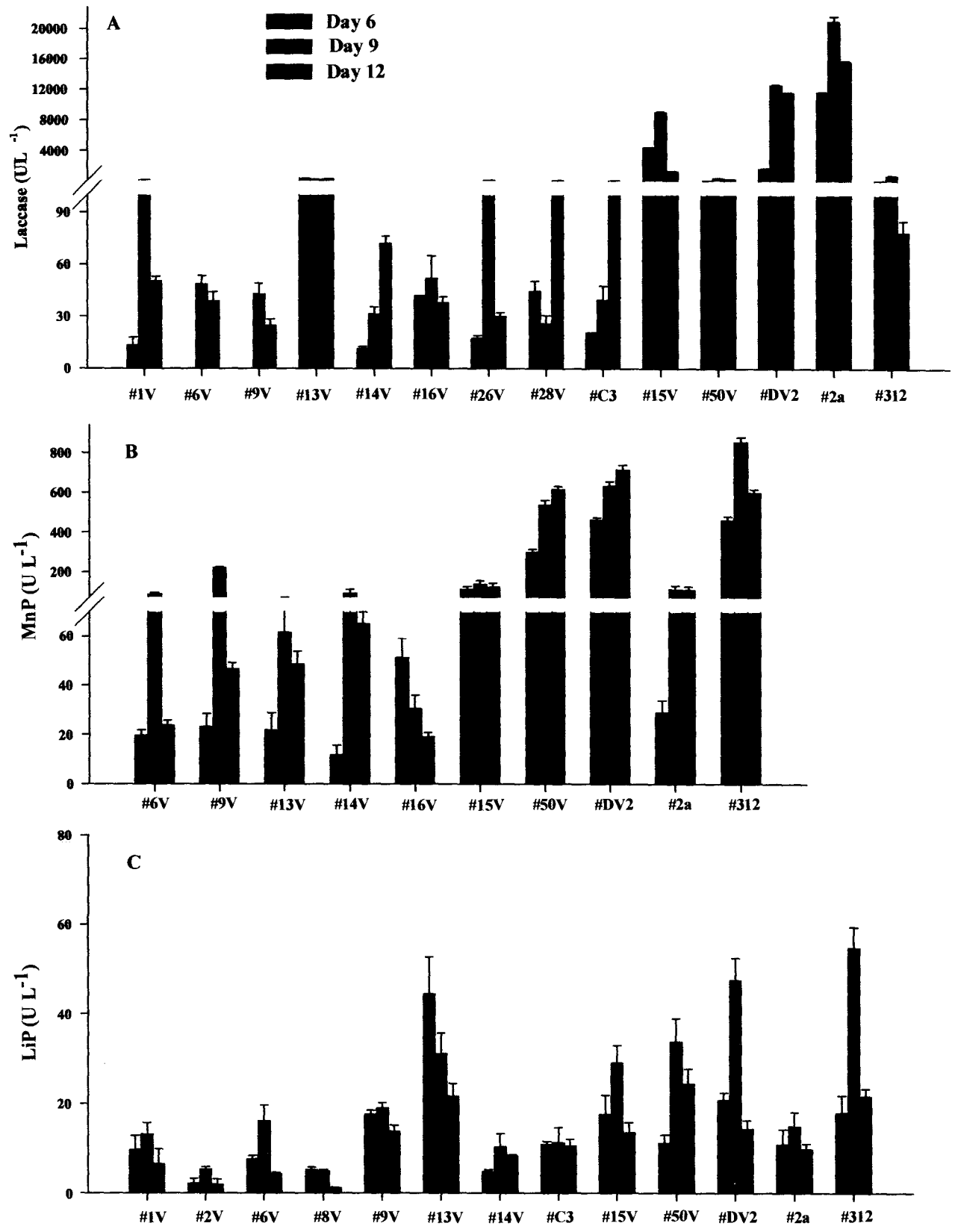
Fig. 2.8: LDE production by several isolates in LN medium. NIOCC #2a and #312 were isolated during previous studies (D'Souza et al., 2006; Raghukumar et al., 1999) and used as reference cultures.
