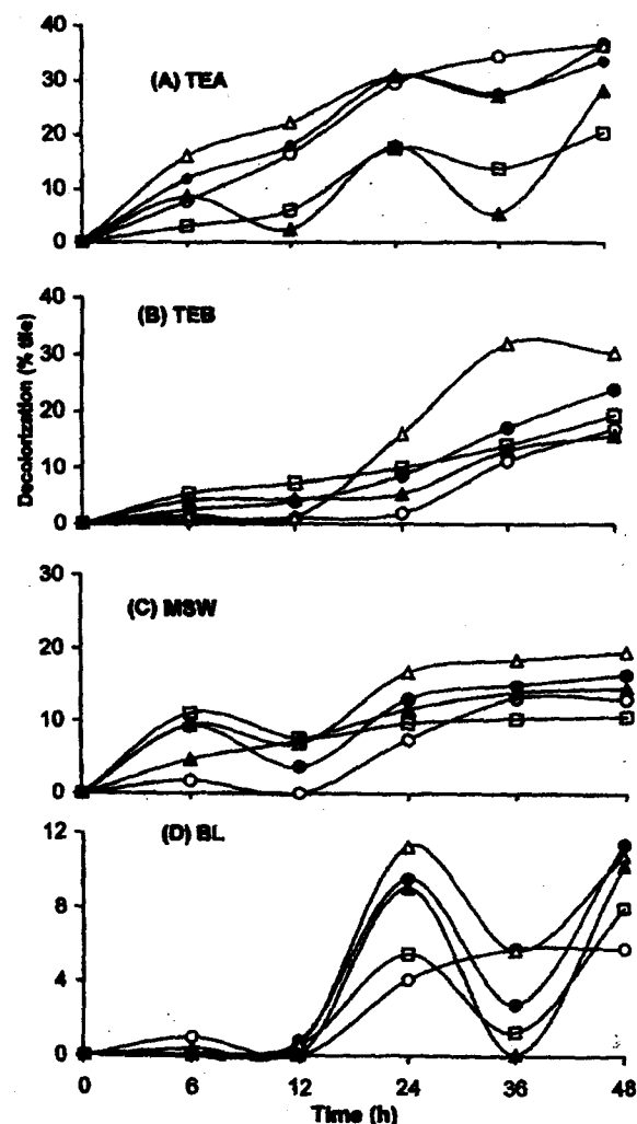
Fig. 1— In vitro decolorization of effluents with 1000 color units each, using 10 U of laccase obtained from different nitrogen sources namely, KNO 3 , glycine, glutamic acid, beef extract and corn steep liquor. Decolorization was monitored from 0 to 48 h. KNO 3 = ○ ; Glycine ● ; Glutamic acid Δ; Beef extract ▲ ; Corn steep liquor □.
