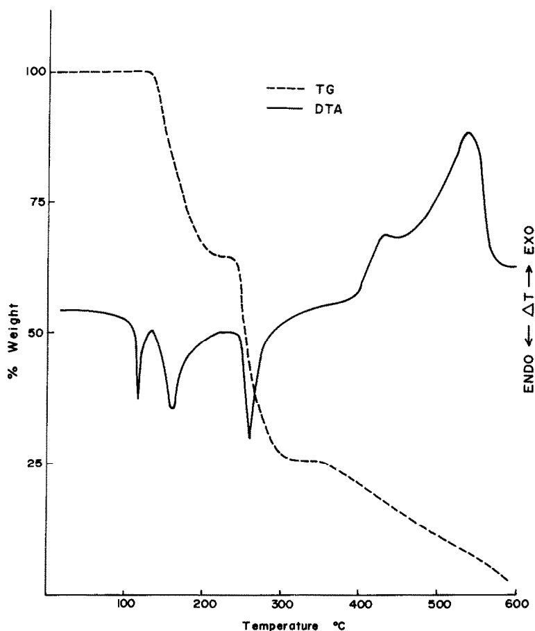
FIG. 1 TG and DTA of N(CH_2COO)_3H(N_2H_5)_2
