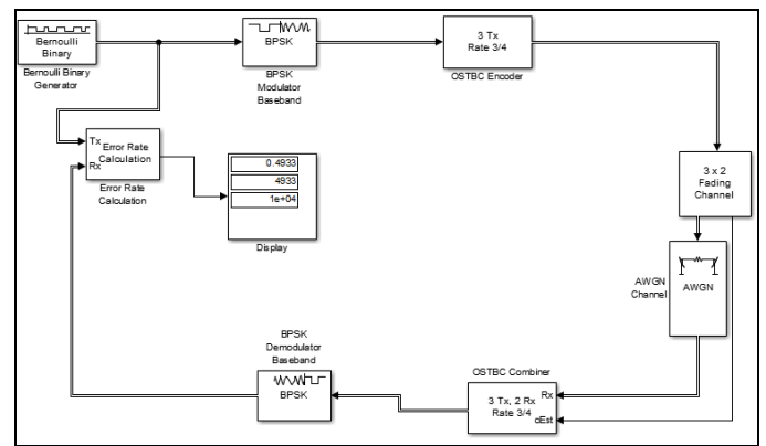
Fig.4.Customized BPSK Modulation Simulink Model
