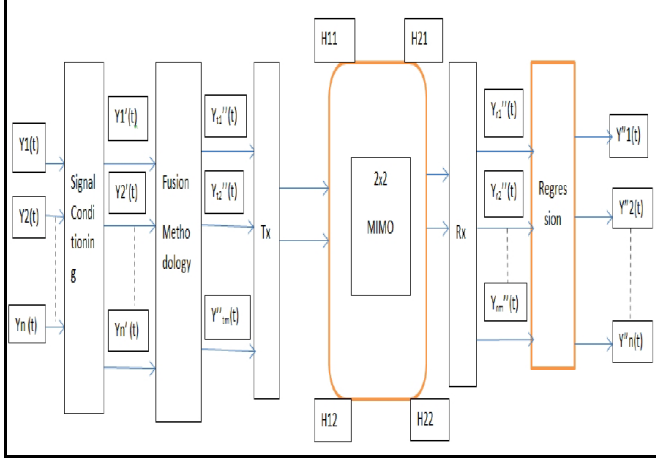
Fig.2.Proposed Architecture For Sensor Data Fusion Over MIMO.
