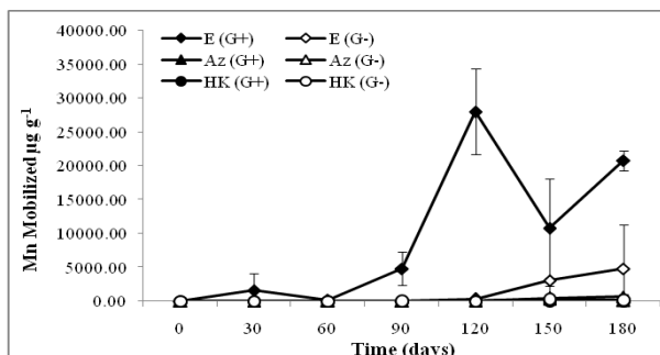
Figure 4. Mobilization rate of Mn from basalt by Bacterial potential isolate R6. The values in the figure are mean values \pm SD, n = 3.
