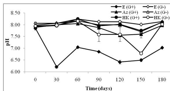
Figure 6. Variation in pH in relation to the mobilization of Mn (E: experiment and Az: azide poisoned control, G+: with added glucose and G-: without added glucose).
