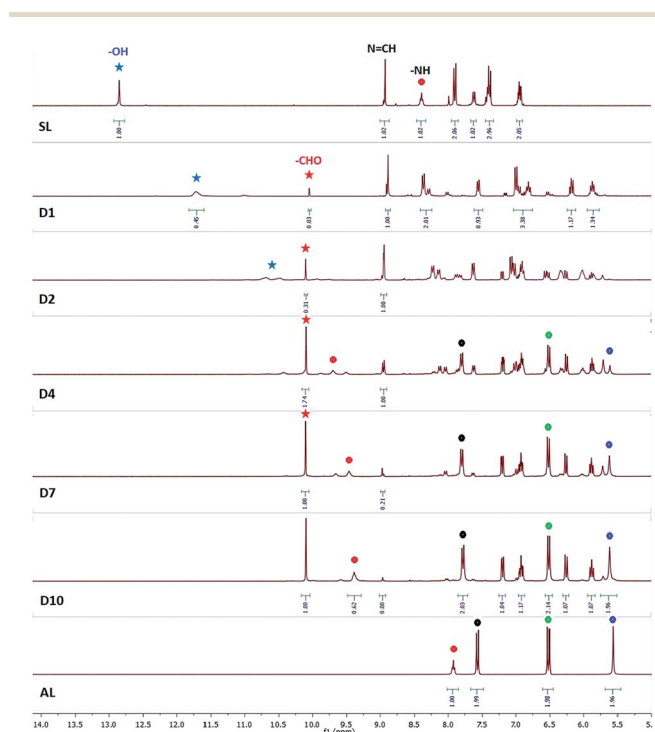
Fig. 1 ^1\text{H-NMR} spectra (DMSO- d_6 ) of SL in the presence of TBAF for 10 days (D1–D10). Signals labelled with red, black, green and blue circles indicate amide -\text{NH} , ortho - \text{CH} , meta - \text{CH} and -\text{NH}_2 protons of AL respectively. Signals labelled with red, and blue stars indicate -\text{CHO} and -\text{OH} protons of salicylaldehyde and SL respectively. (A larger sized version of the spectra with also additional spectra recorded on D3 and D9 is provided in Fig. S20, ESI ^\dagger ).
