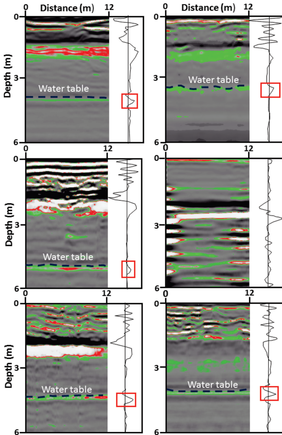
Figure 7. Water table depth from GPR profiles (a) 3.8 m (b) 3.4 m (c) 4.9 m (d) not detectable (e) 4.3 m and (f) 4.1 m.
