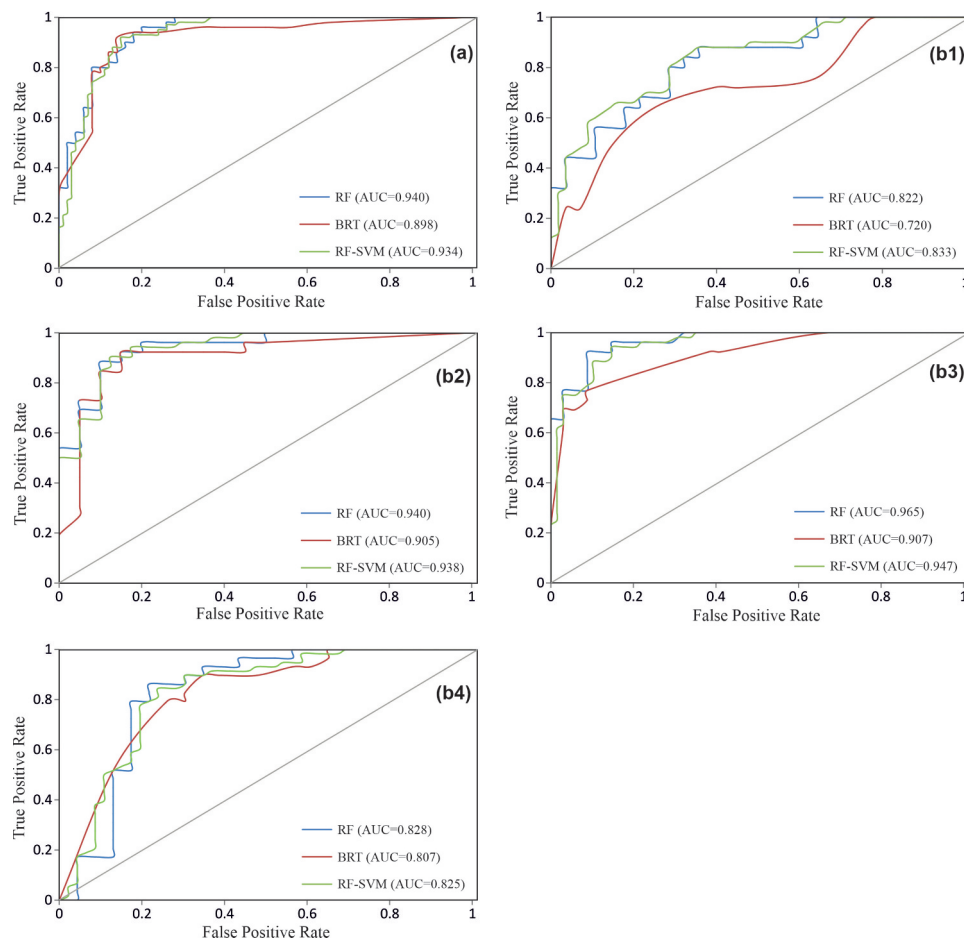
Figure 6. ROC curve of the models in study area (a), secondary areas (b1, b2, b3, b4).
