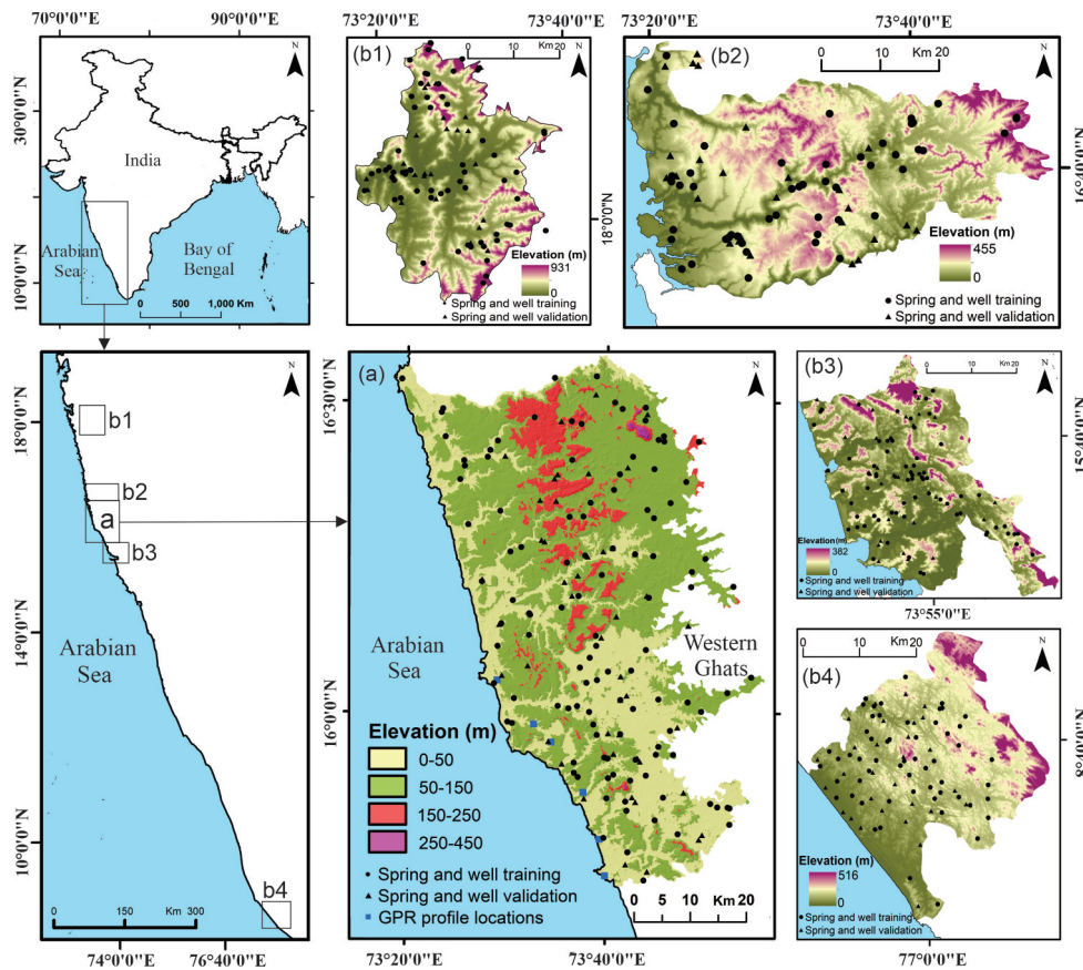
Figure 1. Location maps of the study area (a), and secondary regions (b1, b2, b3, b4).
