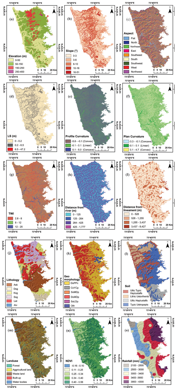
Figure 3. Thematic layers of the groundwater affecting factors (a) elevation, (b) slope, (c) aspect, (d) LS, (e) profile curvature, (f) plan curvature, (g) TWI, (h) distance from rivers, (i) distance from lineaments, (j) lithology, (k) geomorphology, (l) soil, (m) land use, (n) NDVI, (o) rainfall.
