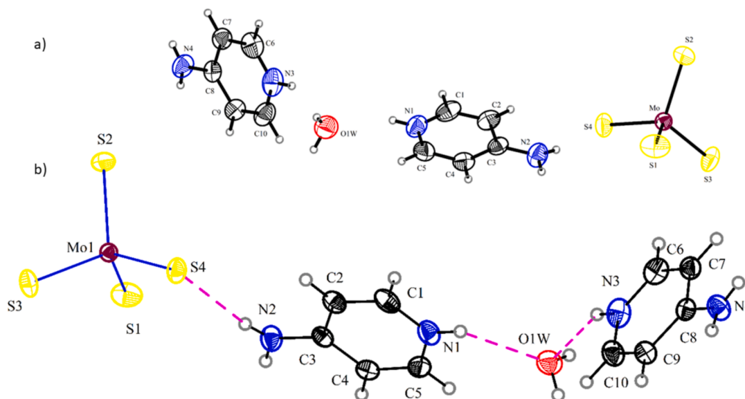
Fig. 1. a) Crystal structure of (4\text{-aminopyridinium})_2[\text{MoS}_4]\cdot\text{H}_2\text{O} 1 showing atom labeling scheme. The thermal ellipsoids are drawn at 30 % probability, and the H atoms are shown as circles with an arbitrary radius. b) Intramolecular hydrogen bonds are shown in purple dotted lines in 1.
