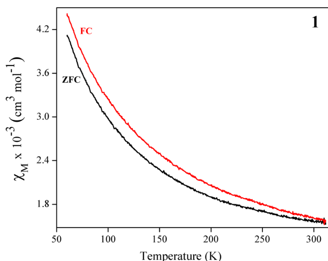
Figure 8. Plot of zero-field-cooled (ZFC)–field-cooled (FC) magnetic susceptibility for 1 as a function of temperature under an applied field of 100 G between 60 and 310 K.
