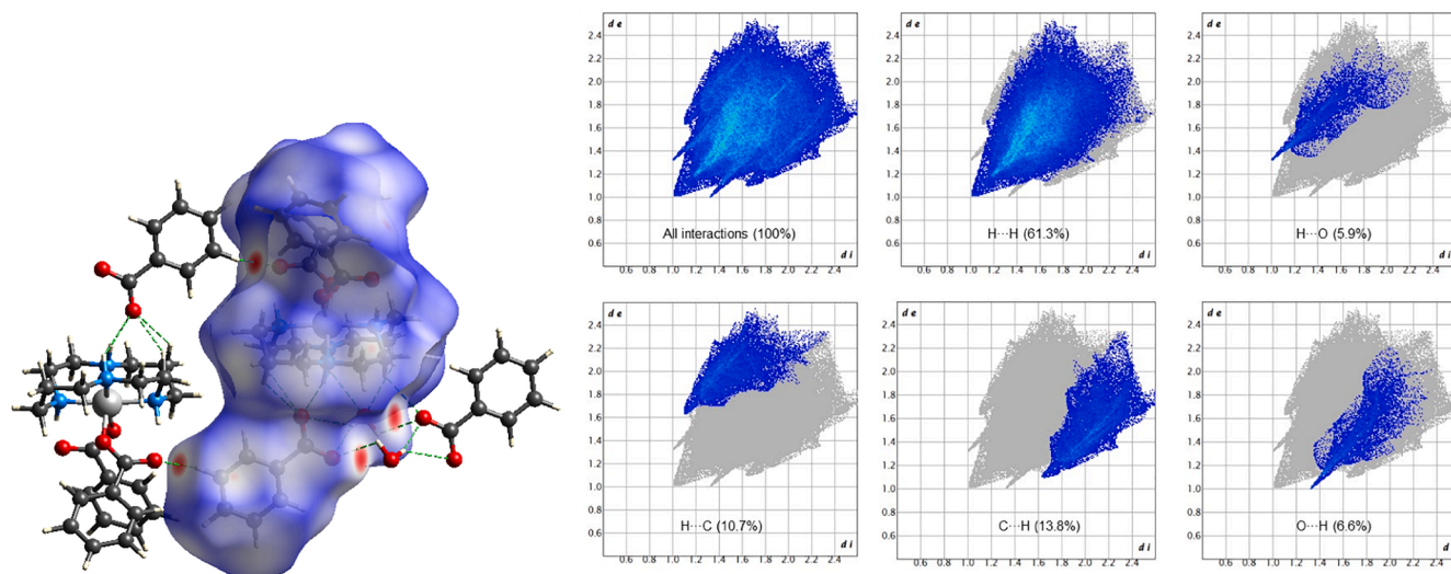
Fig. 4. a) HS mapped with the d_{\text{norm}} function for 1 showing the intermolecular interactions. b) 2D fingerprint plots with the relative contribution in % of interaction to HS area.
