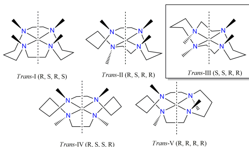
Figure 1. Shows the trans conformers of the cyclam ligand
