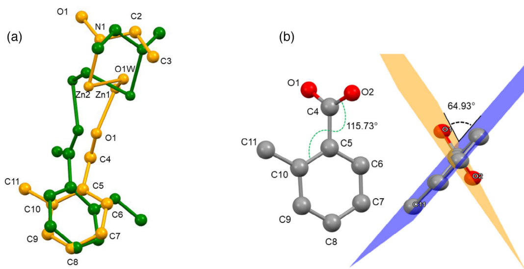
Figure 4. (a) Overlay diagram of the asymmetric units of 1 (yellow) and 2 (green) compounds with rmsD = 1.9347 and max = 3.711 Å. (b) View along the carboxylate anion highlighting the orientation of the substituents (left) and dihedral angle between the mean plane through benzene ring (C5-C6-C7-C8-C9-C10) and (O1-C4-O2) (right).
