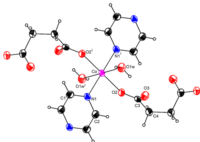
Figure 3. Crystal structure of [Co(H 2 O) 2 (pyz)(suc)] ( 2 ), showing the thermal ellipsoids drawn at the 50% probability level for all of the atoms except for the H atoms that are shown as spheres of arbitrary radii. Symmetry code: (i) -x + 3/2, -y + 3/2, -z + 1 .
