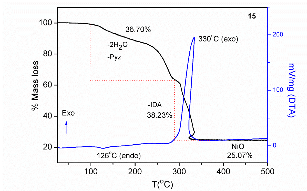
Figure 8. The TG-DTA plot of compound 15 .
