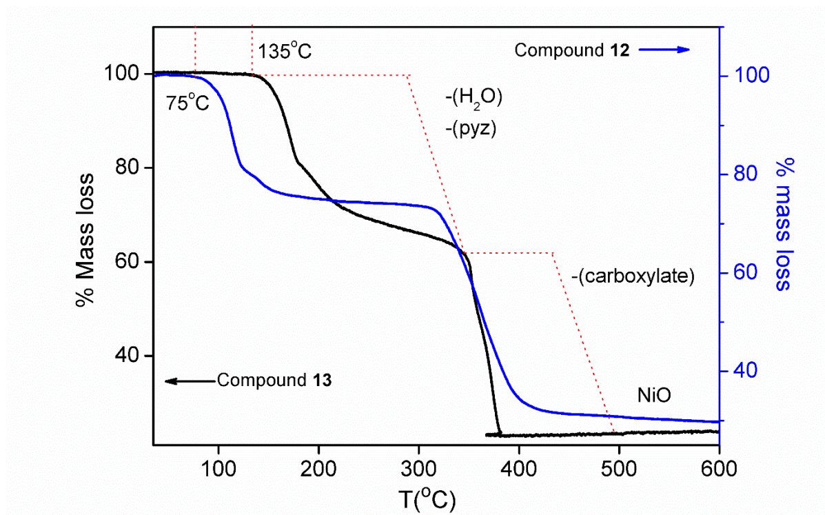
Figure 6. The overlaid TG curves of compounds 12 (blue) and 13 (black).
