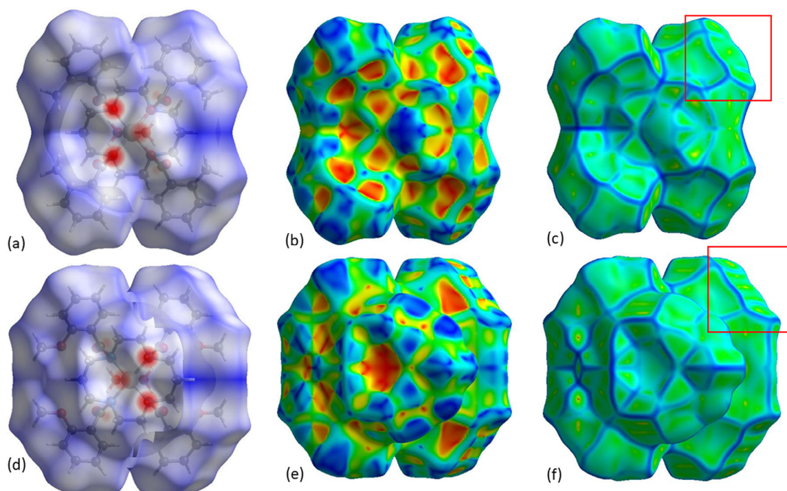
Figure 6. Hirshfeld surface mapped with (a) d_{\text{norm}} ranging from -0.40 Å (red) to 2.04 Å (blue) (b) shape index, and (c) curvedness of 1 and (d) d_{\text{norm}} ranging from -0.47 Å to 1.74 Å (e) shape index, and (f) curvedness of 2 (view along a-axis).
