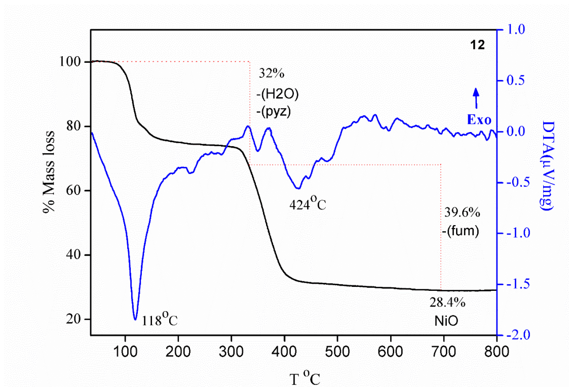
Figure 5. The TG-DTA plot of compound 12.
