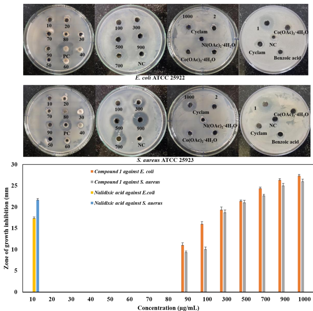
Figure 22 Antibacterial activity of 1 at different concentrations (10, 20, 30, 40, 50, 60, 70, 80, 90, 100, 300, 500, 700, 900 and 1000 μg/ml); NC, negative control (DMSO: H 2 O); PC, positive control (Nalidixic acid, 10 μg/ml); 2 , [Ni(cyclam)(H 2 O) 2 ](MeOBz) 2 ·4H 2 O.
