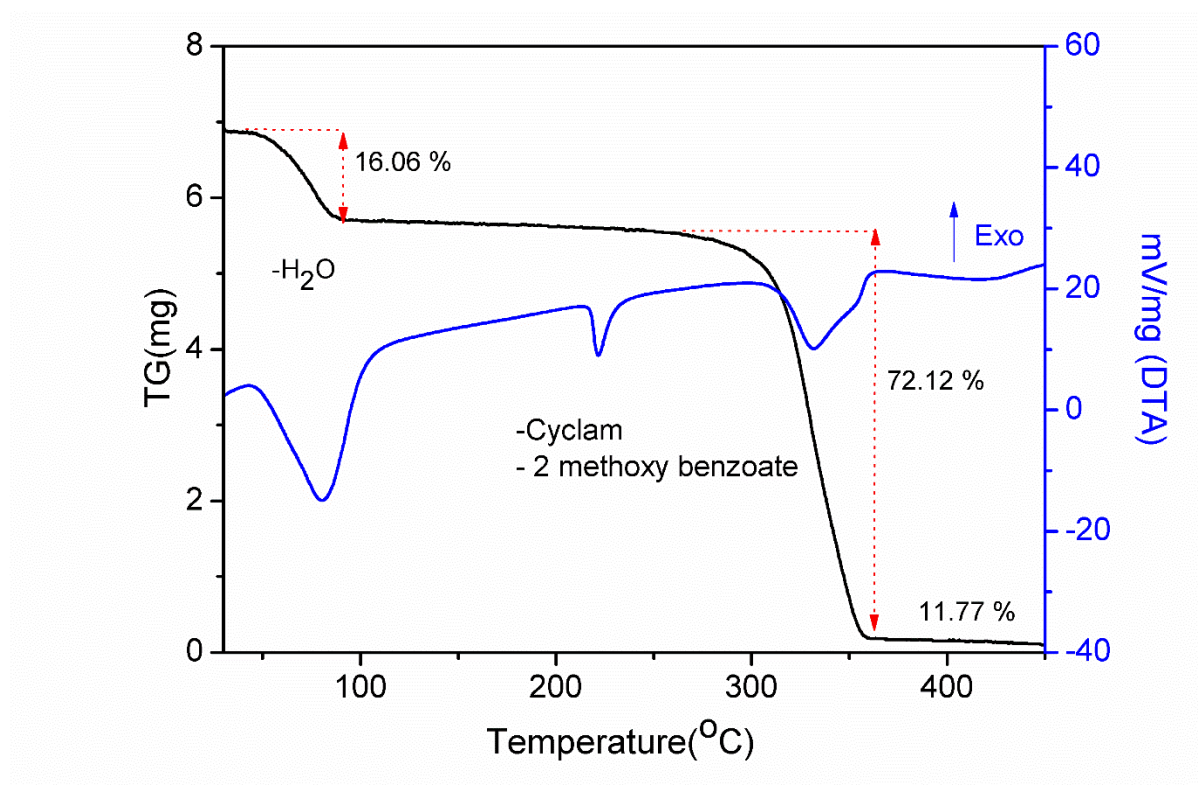
Figure 16 The TG-DTA plot of trans -[Ni(cyclam)(H 2 O) 2 ](MeOBz) 2 ·4H 2 O in N 2 atmosphere.
