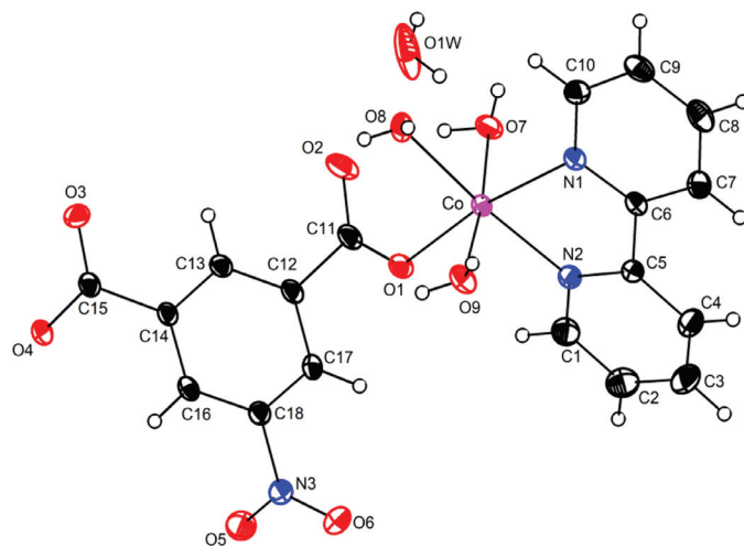
Fig. 10. Crystal structure of [\text{Co}(\text{H}_2\text{O})_3(\text{bpy})(\text{nip})]\cdot\text{H}_2\text{O} 2 showing the thermal ellipsoids drawn at the 50% probability level for all of the atoms except for the H atoms that are shown as spheres of arbitrary radii.
