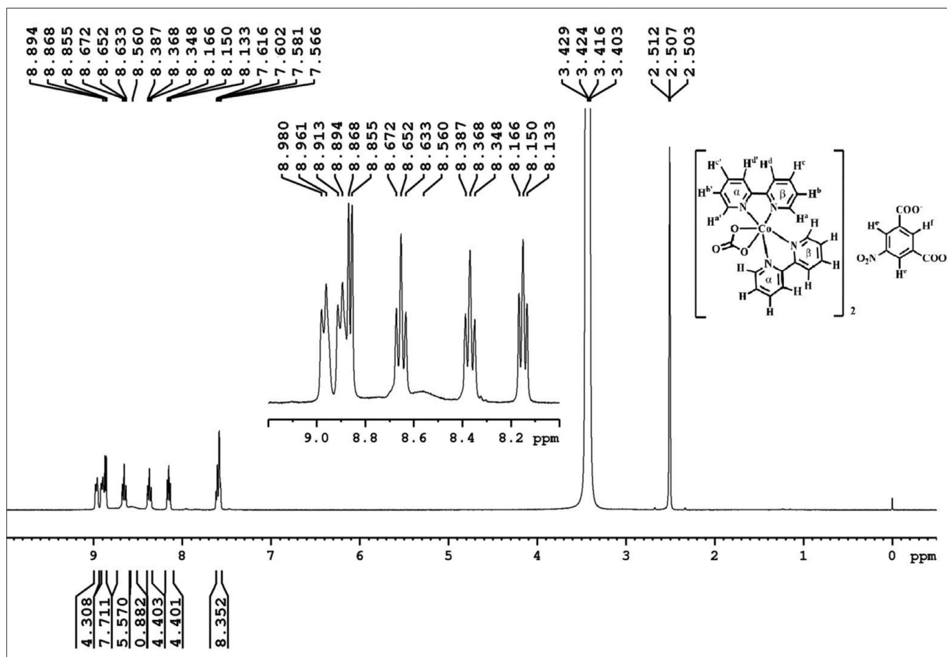
Fig. 4. 1 H-NMR spectrum of [Co(bpy) 2 (CO 3 )] 2 (nip)·11H 2 O ( 1 ) recorded in solvent CD 3 OD.
