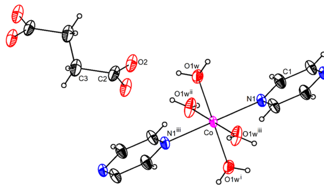
Figure 5. Crystal structure of [Co(H 2 O) 4 (pyz)](suc) ( 3 ) showing the thermal ellipsoids drawn at the 50% probability level for all of the atoms except for the H atoms that are shown as spheres of arbitrary radii. Symmetry code: (i) -x + 1, -y + 1, -z + 1 (ii) x, y, -z + 1 (iii) -x + 1, -y + 1, z .
