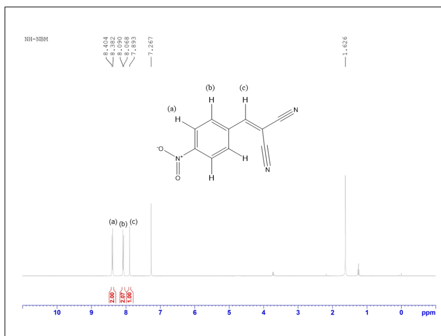
Figure 32. 1 H-NMR data for (3a) (400 MHz, CDCl 3 , IIT-Goa); (a) \delta 8.4 (2H, d, ArH), (b) \delta 8.09 (2H, d, ArH), (c) \delta 7.89 (1H, s, =CH)
