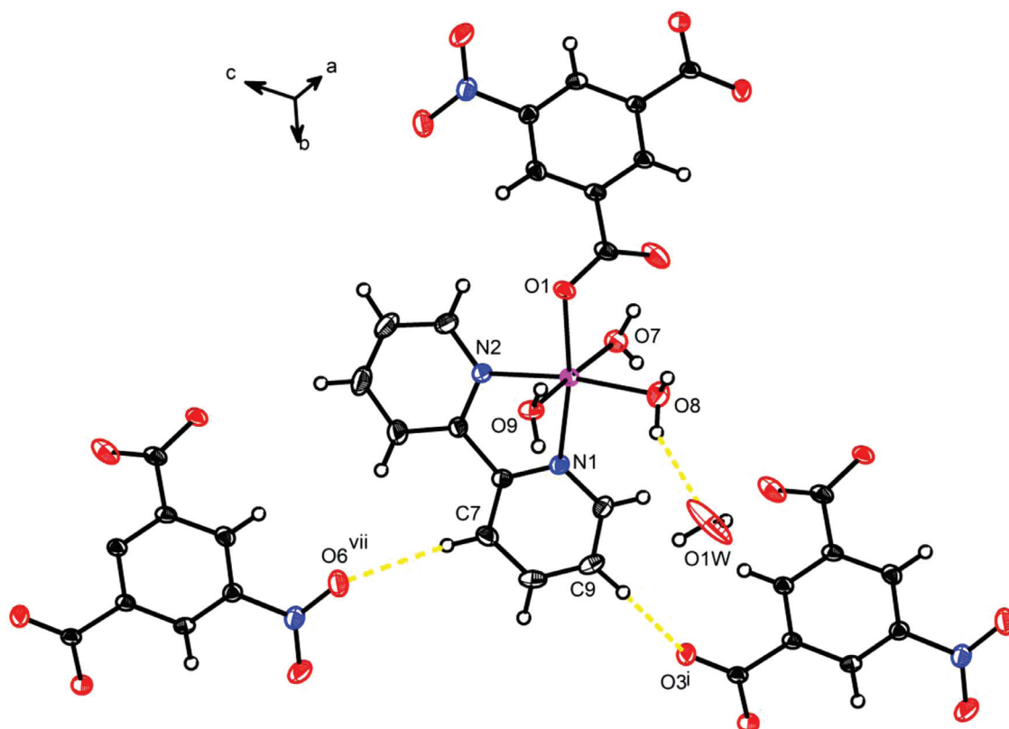
Fig. 11. The intramolecular H-bonding between O-H...O and C-H...O in 2 shown as broken lines (Yellow). Symmetry code: (i) -x + 1, -y + 1, -z + 1 (vii) x - 1, y + 1, z (For interpretation of the references to color in this figure legend, the reader is referred to the web version of this article.).
