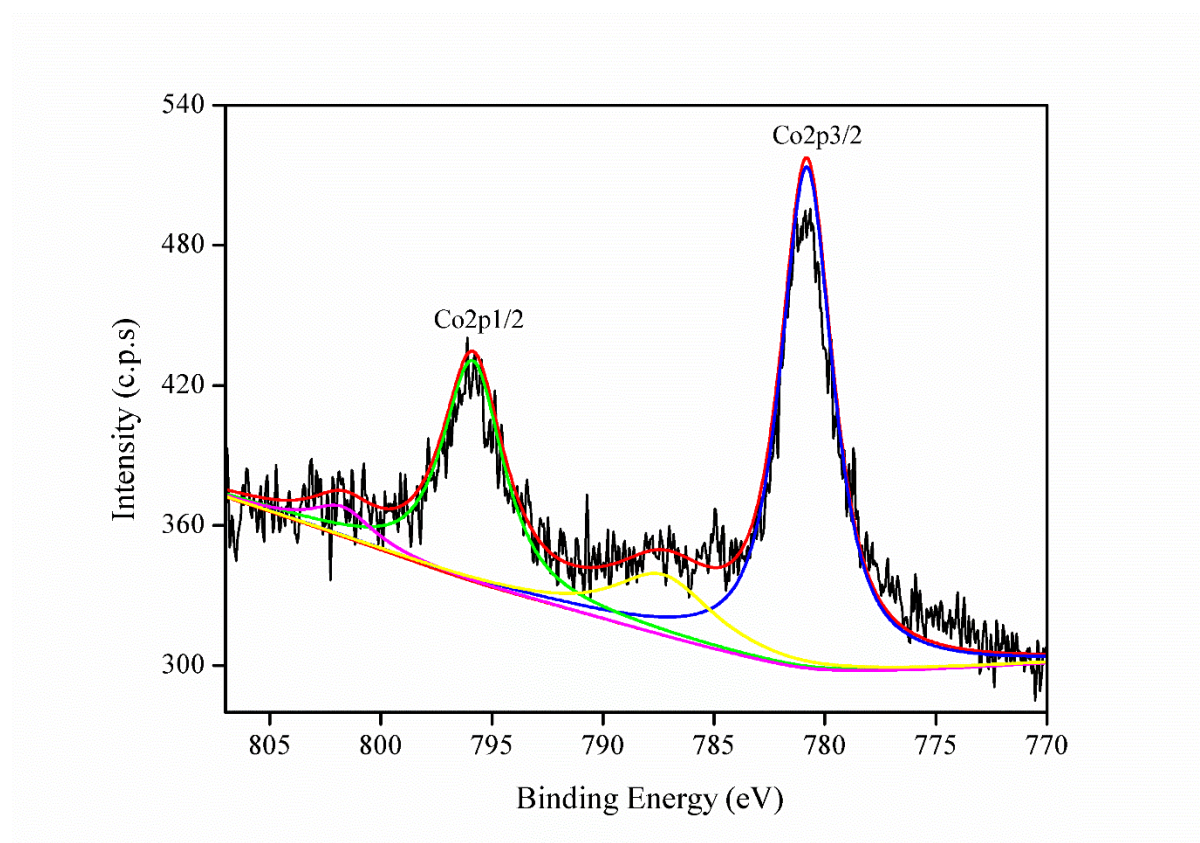
Figure 5. The XPS spectrum of compound 1.
