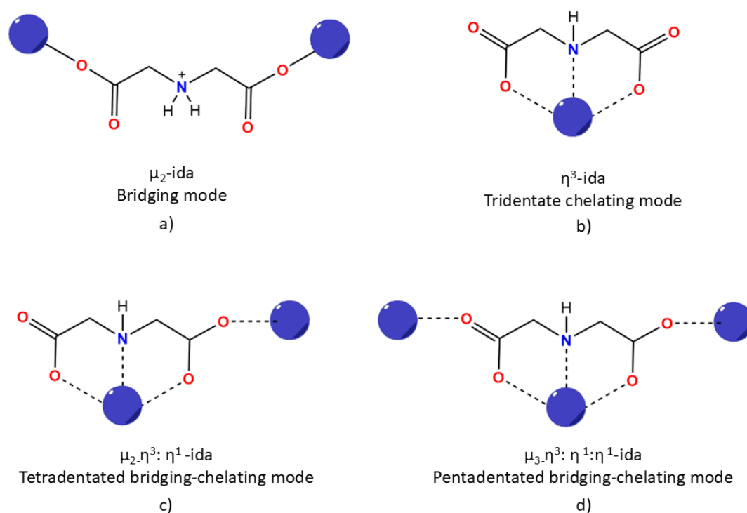
Figure 18. Schematic representation of the coordination modes of \text{ida}^{2-} anion with metal ions.
