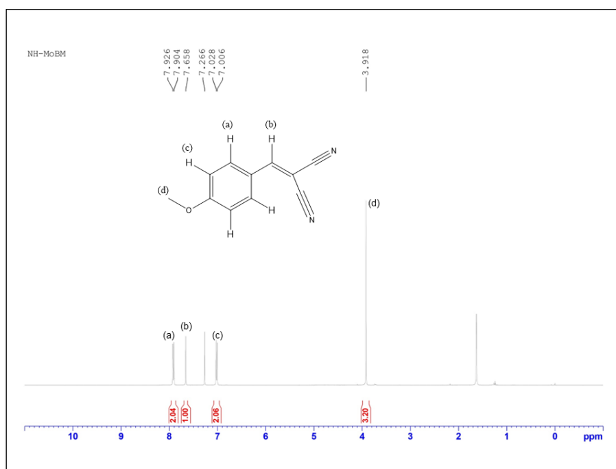
Figure 33. 1 H-NMR data for (4a) (400 MHz, CDCl 3 , IIT-Goa); (a) \delta 7.92 (2H, d, ArH), (b) \delta 7.66 (1H, s, =CH), (c) \delta 7.03 (2H, d, ArH) and (d) \delta 3.92 (3H, s, OCH 3 ).
