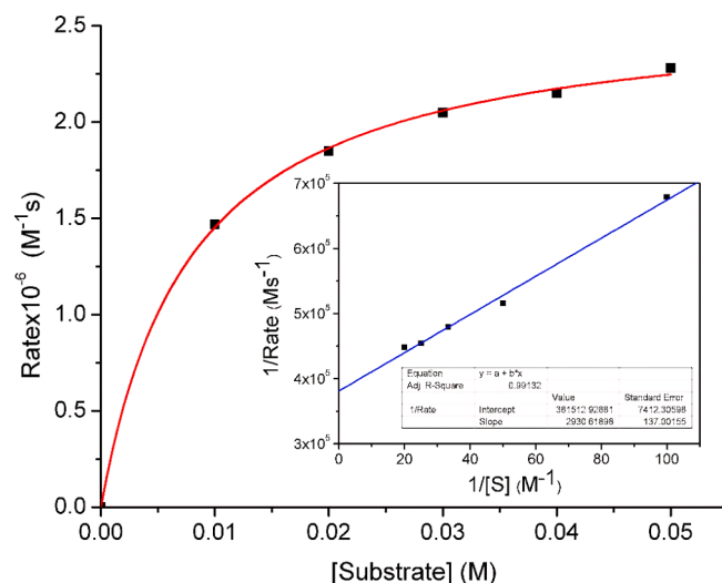
Fig. 8. The plot of the initial rates versus substrate concentration. The inset shows the Lineweaver-Burk plot.
