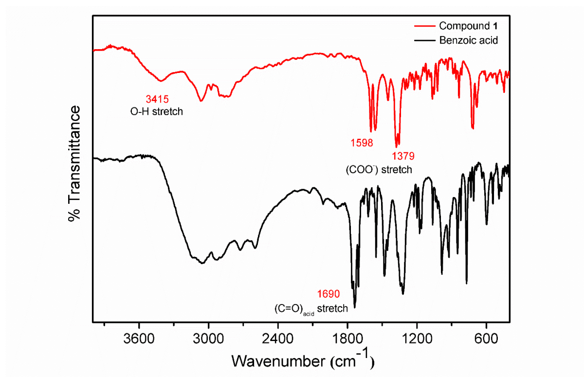
Figure 1 The infrared spectra of compound 1 overlaid with that of benzoic acid.
