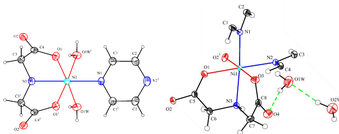
Figure 9. The portion of 0D and 3D structures showing octahedral coordination in hydrate isomers 14 (Left), symmetry code, and 15 (Right)
