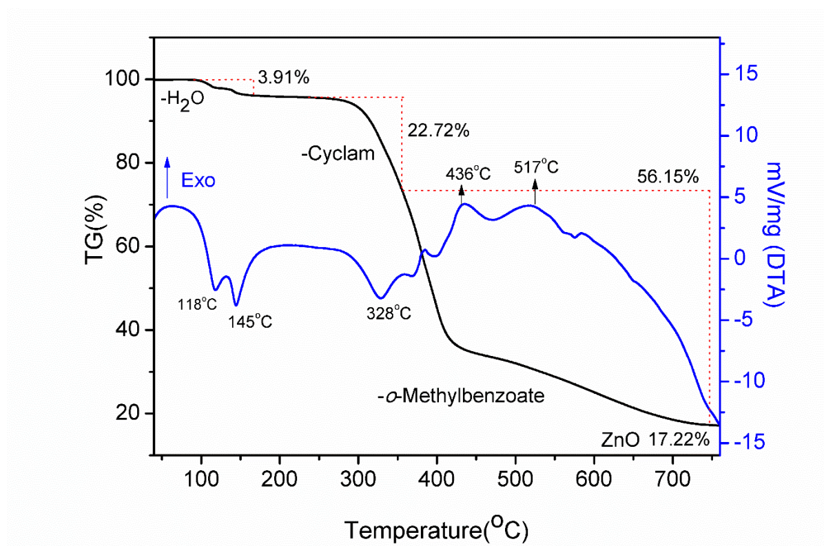
Figure 4. The TG-DTA plot of 4 recorded at a heating rate of 10 °C min -1 in N 2 atmosphere
