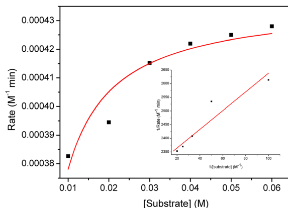
Fig. 5 Plot of initial rates versus substrate concentration from the oxidation of 3,5-DTBC catalyzed by 1 . The inset shows the Lineweaver-Burk plot.
