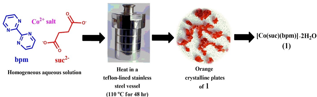
Scheme 1. Synthetic methodology for compound 1.
